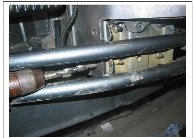
Figure 4 – Driver's side shown. Use 10mm long drill bit as required.
