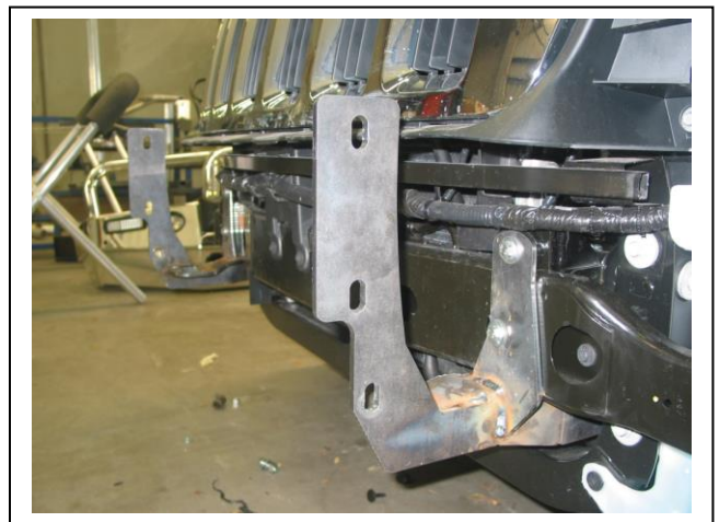
Figure 6: ECB steel mounting brackets fitted. Bumper removed for photo.
