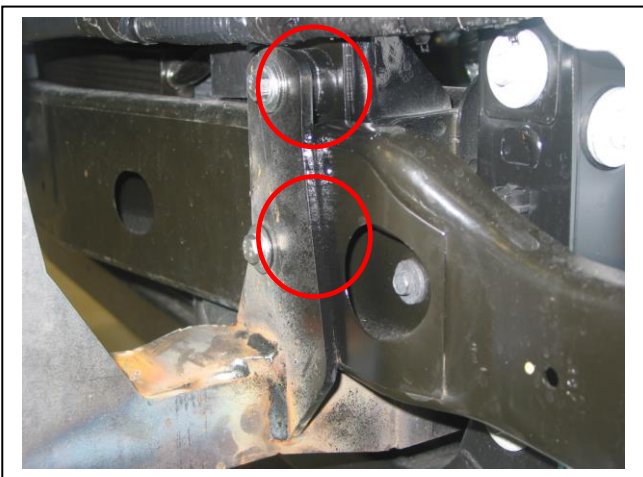
Figure 5: ECB steel mounting brackets showing spacer placement
