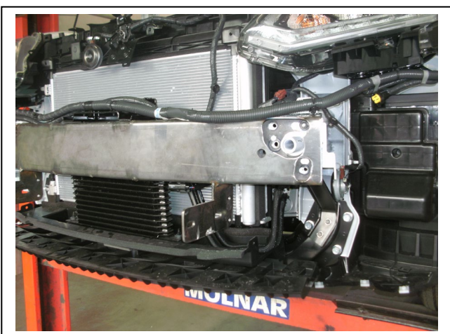
Figure 5: ECB Steel mounting bracket fitted.
