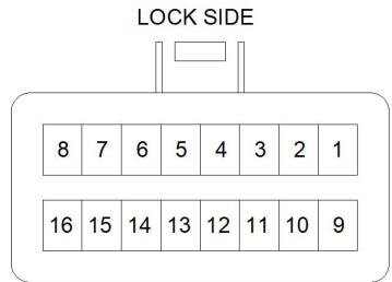
VEHICLE CONNECTOR
